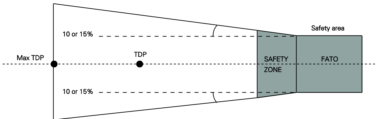
Figure 2: Obstacle accountability
