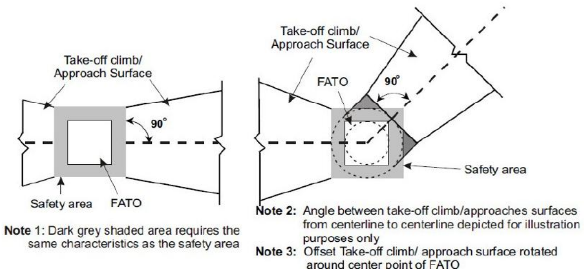
Figure 4-1: Obstacle limitation surfaces - take-off climb & approach surface
