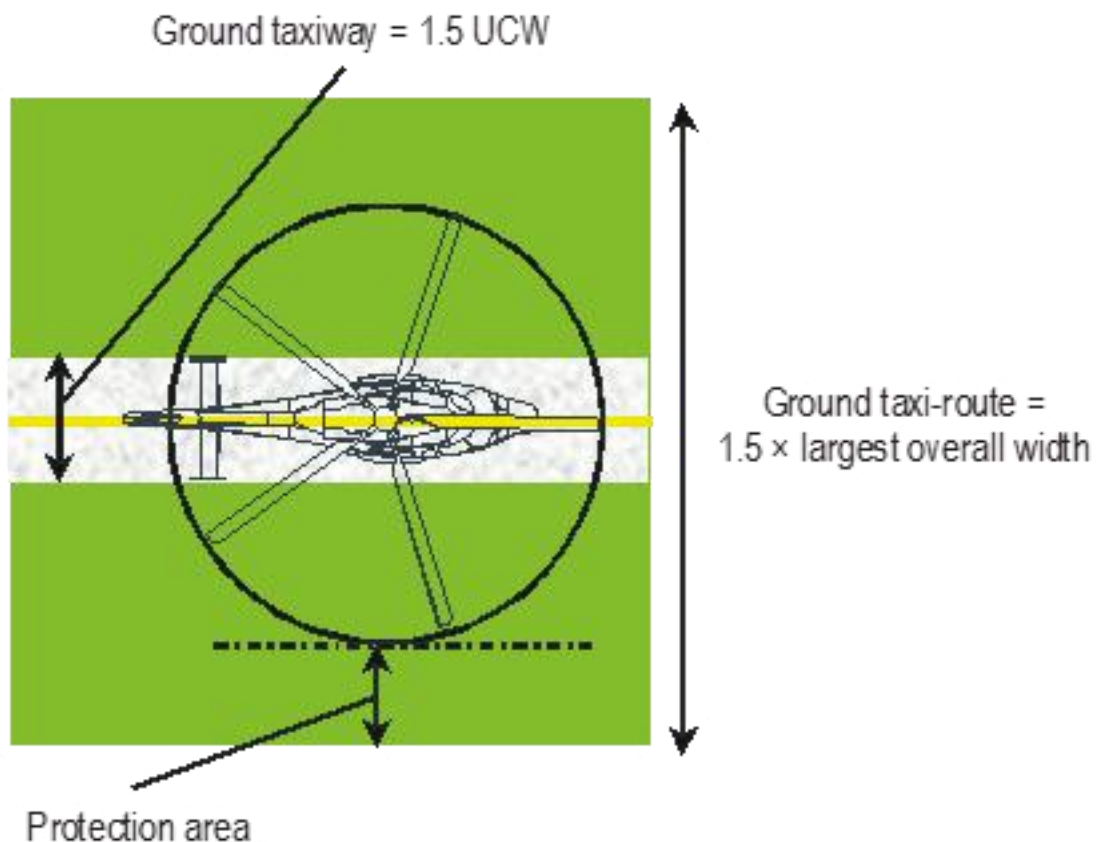
Figure E-2: Helicopter air taxi-route / taxiway
