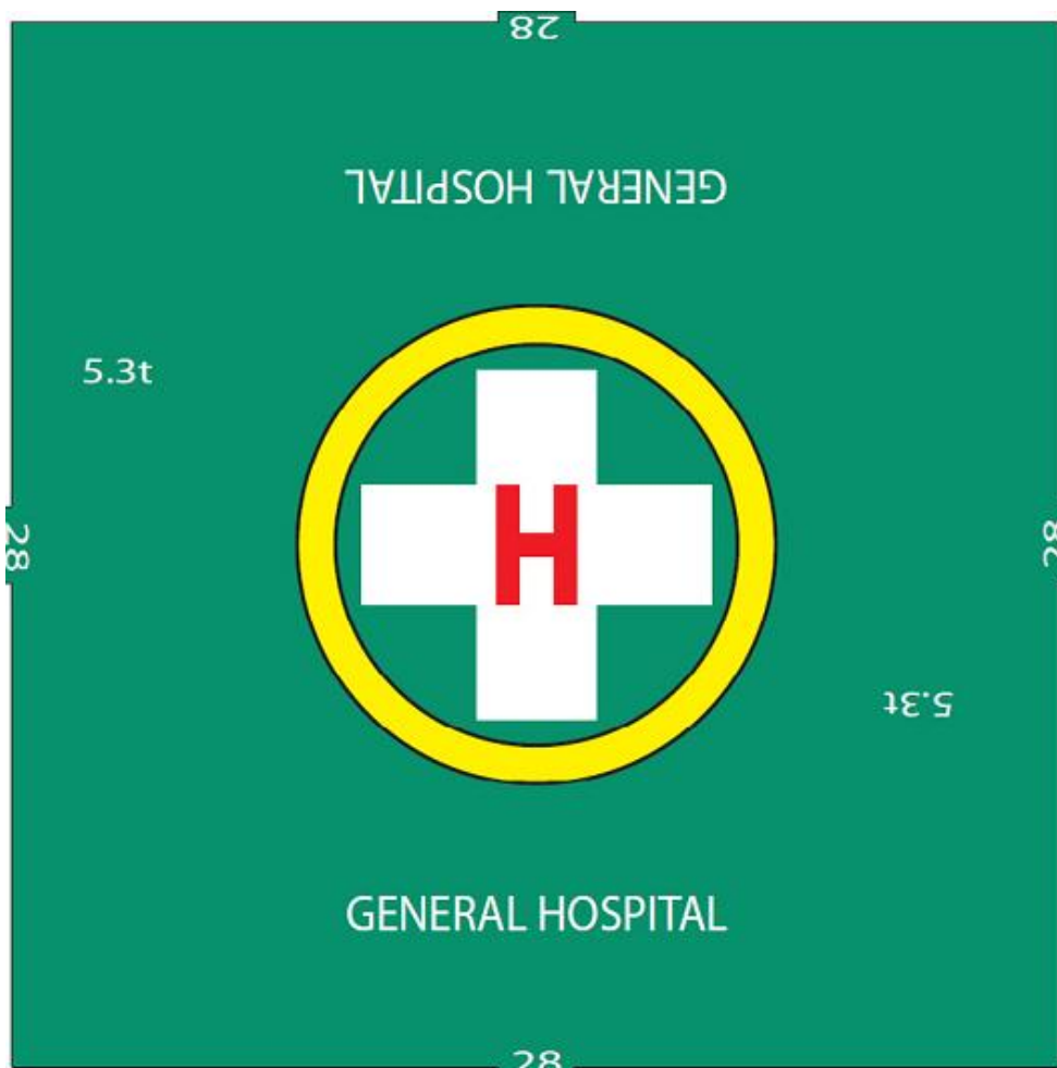
Figure 6: Markings for single main rotor helicopters (hospital)
