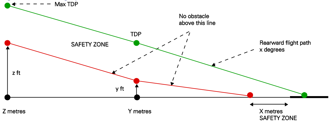
Figure 1: Rearward flight path
